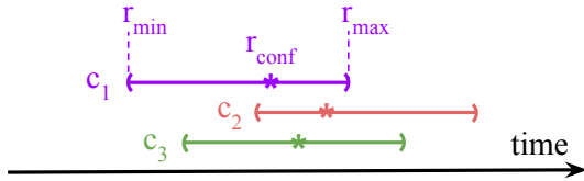
Fig. 2: The same transaction in the view of three different pod clients. Each client assigns it a minimum round r_{\min} and a maximum round r_{\max} . If it gets confirmed, the confirmation round r_{\text{conf}} will be between these two values. The r_{\text{conf}} that each client locally computes respects the bounds of each other client.
